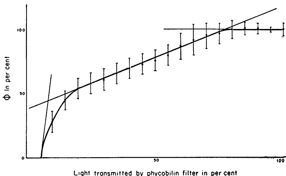
FIGURE 5 Relation between the proportion of incident white light transmitted by mixed phycobilin filters of various optical densities, and the relative quantum yield.
